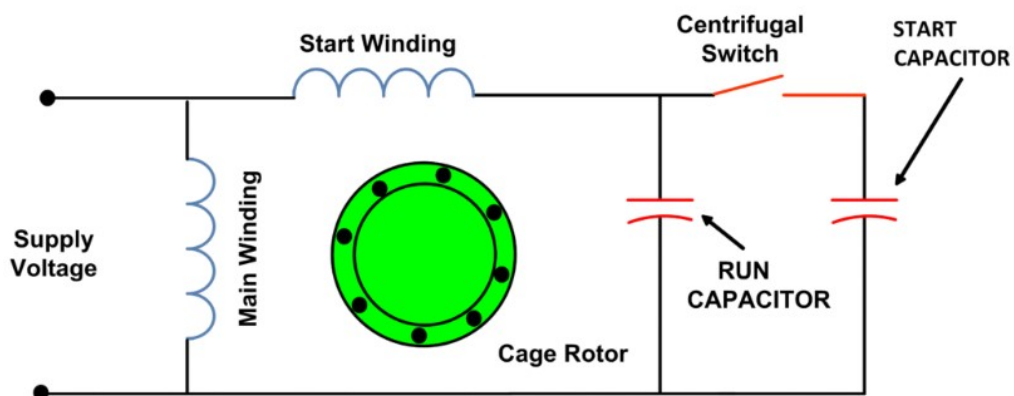
Fig.12: Capacitor Start and Capacitor Run Motor
